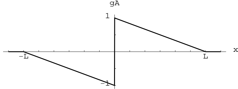
Fig.1: the DLCQ function g_A(x^-) .
